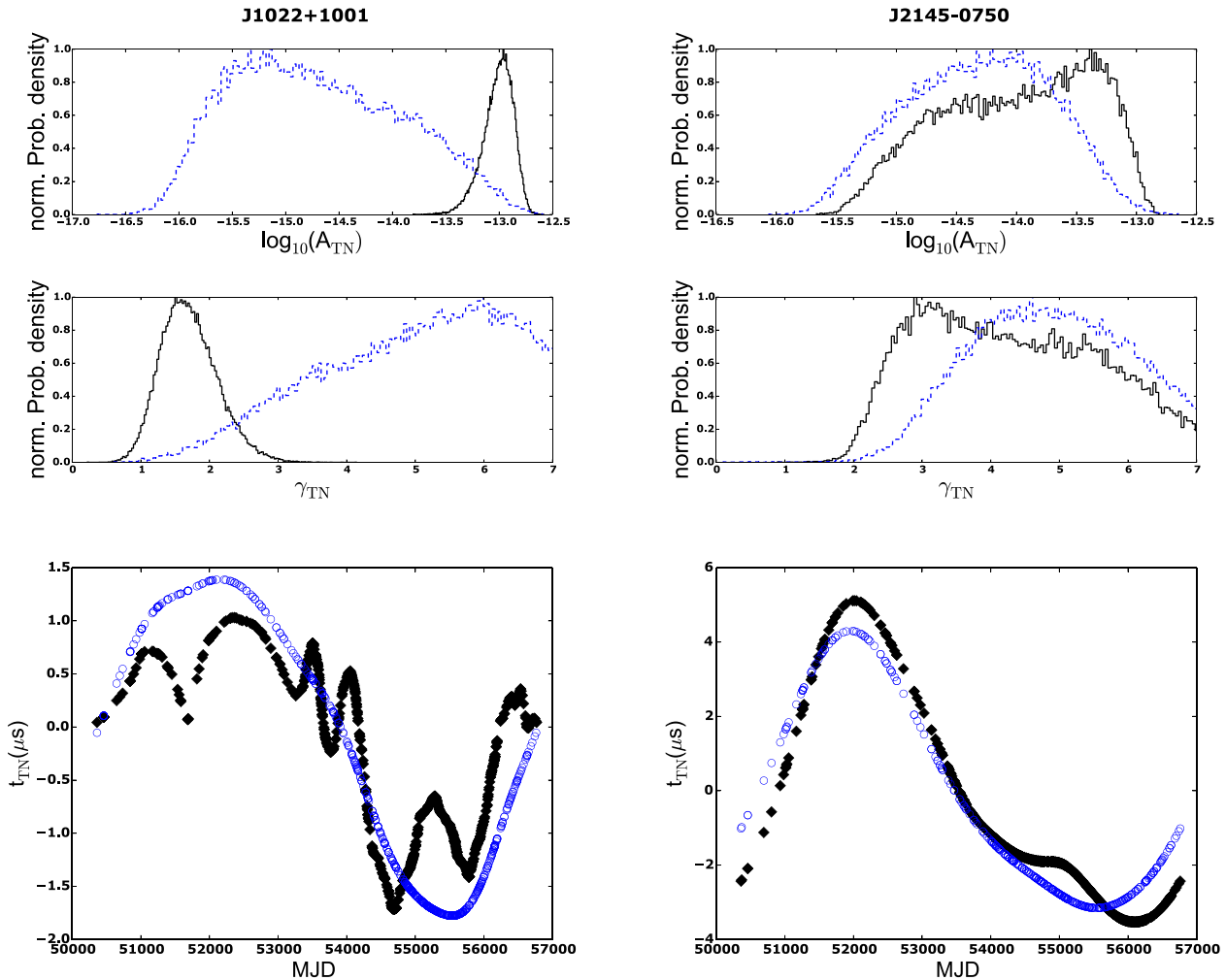
Figure 6. Top panel: comparison of the one-dimensional marginalized PPDs of the TN parameters when using the full EPTA data set (solid, black lines) and the data subset which does not include any NRT-BON data (blue, dashed lines). Bottom panel: comparison of the TN waveforms ( t_{\text{TN}} ) when performing the noise analysis on the full EPTA data set (filled black diamonds) and the data subset which excludes the NRT-BON data (open blue circles). See Section 5 for a discussion.
